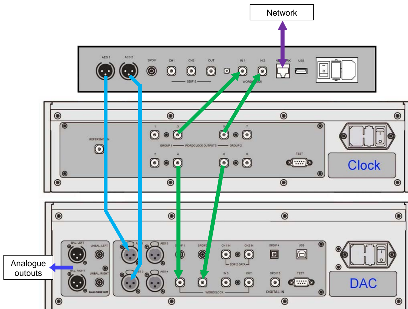
Figure 3 – Using the Network Bridge with a Vivaldi DAC and Master Clock
