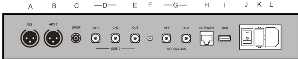
Figure 4 – Rear panel
